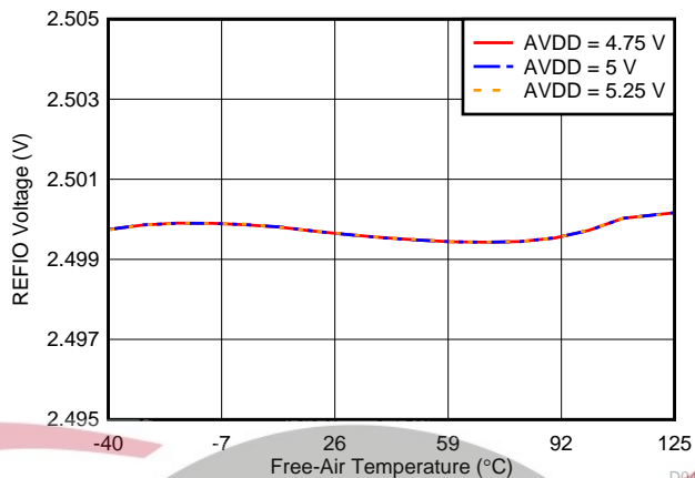
Figure 60. Variation of Internal Reference Output (REFIN/REFOUT) vs Supply and Temperature
