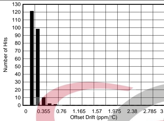
Figure 22. Offset Drift Histogram Distribution ( \pm 10\text{ V} )
